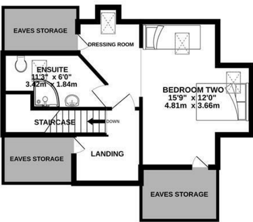
2ND FLOOR 356 sq.ft. (33.1 sq.m.) approx.
